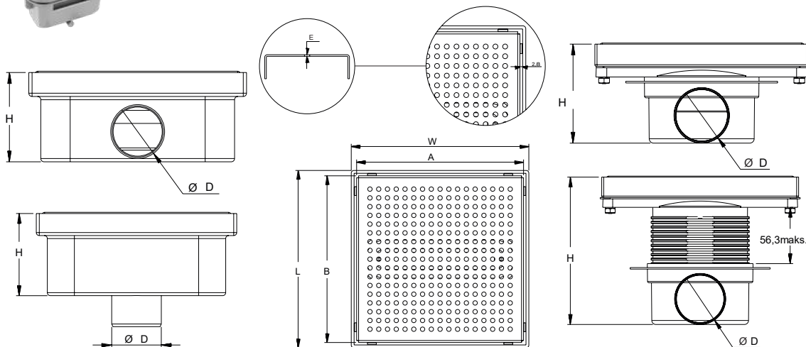
HM-31363
