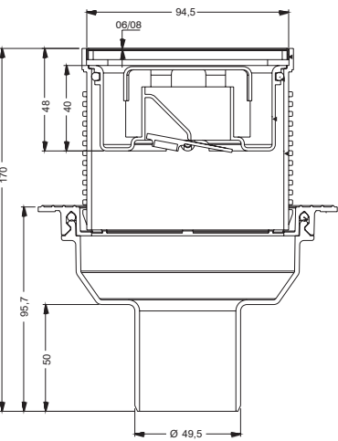
Ø 50 VERTICAL OUTLET
